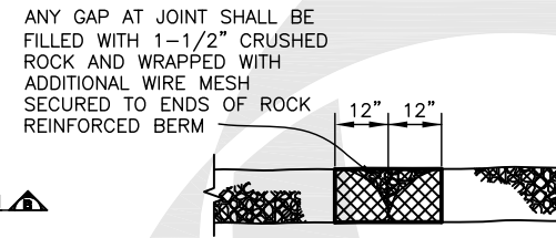
JOINT DETAIL SCALE: 1/2" = 1'-0"
